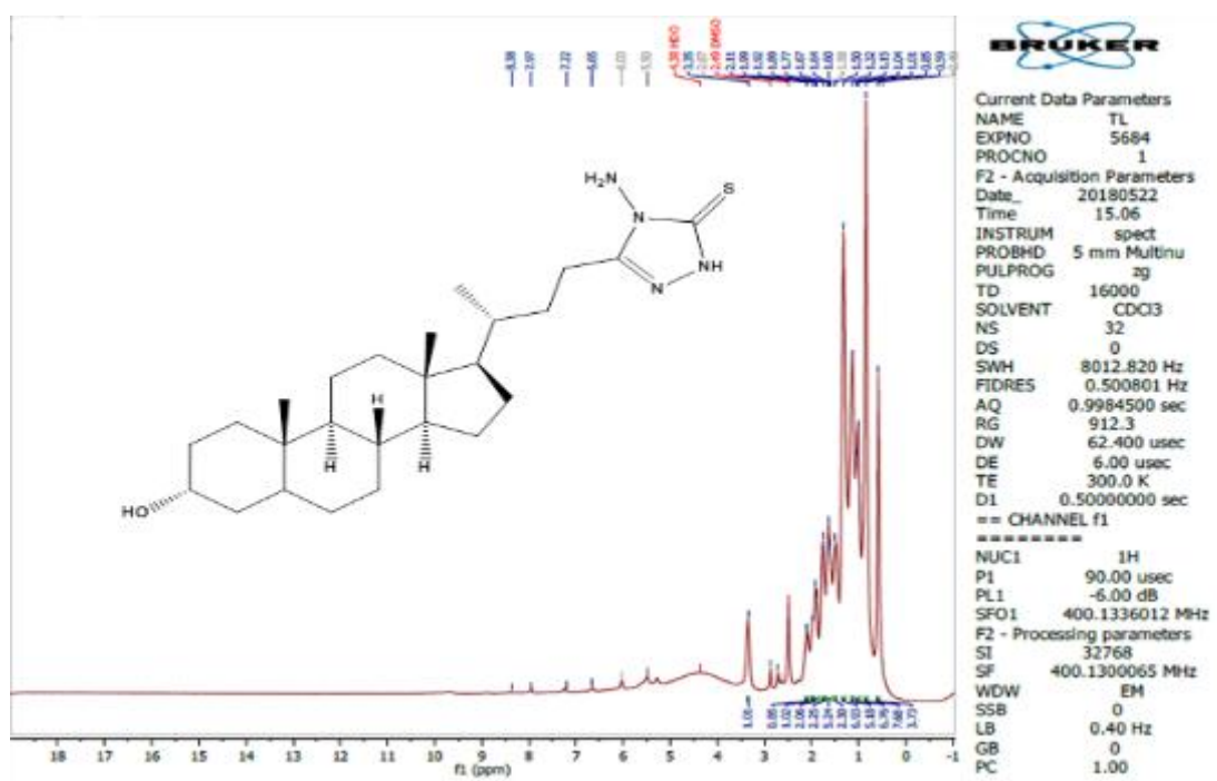
Fig (7) 1 HNMR - spectrum of prepared TL
